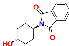
2-(Trans-4-hydroxycyclohexyl)-1H-isindole-1,3(2H)-dione
