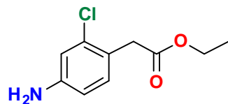
Ethyl 2-(4-amino-2-chlorophenyl)acetate
