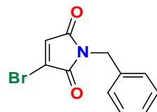
1-Benzyl-3-bromo-1H-pyrrole-2,5-dione
