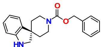
1'-N-Cbz-1,2-dihydro-1'-H-spiro[indole-3,4'-piperidine]
