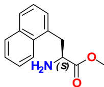
(S)-Methyl 2-amino-3-(naphthalen-1-yl)propanoate
