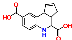
3a,4,5,9b-Tetrahydro-3H-cyclopenta[c]quinoline-4,8-dicarboxylic acid (CCX 1959)
