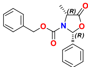
(2R,4R)-3-Benzyloxycarbonyl-4-methyl-2-phenyl-1,3-oxazolidin-5-one
